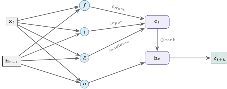
Figure 4: Simplified schematic of a single LSTM cell used to forecast the inter-bank rate spread \delta_{t+h} . Gates f, i, o are sigmoid activations; \tilde{c} uses tanh. See equations (28)–(34).
