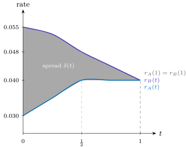
Figure 2: Illustrative rate paths for Banks A and B over [0, 1] . The shaded region represents the exploitable spread \delta(t) = r_B(t) - r_A(t) . Both rates are plotted in natural coordinates scaled linearly to the drawing canvas; no inverse scaling is applied to node text. Rates converge at t = 1 by Assumption 2.2 (ii).
